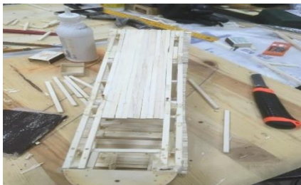
Fig. 14. Reinforcements of the Lower Bridge Structure
